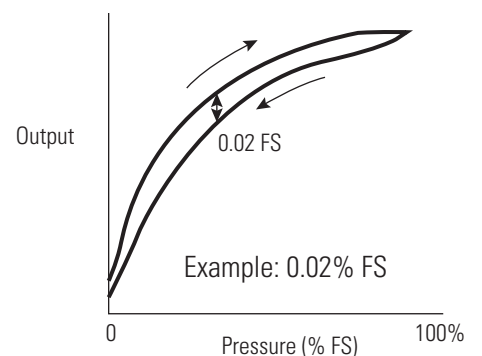
Figure 6. Hysteresis
