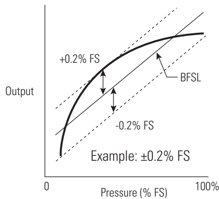
Figure 5. Linearity
