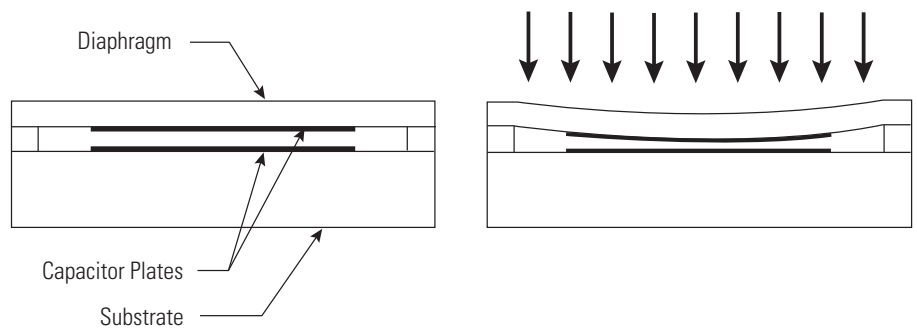
Figure 1. Capacitive Sensing Element
