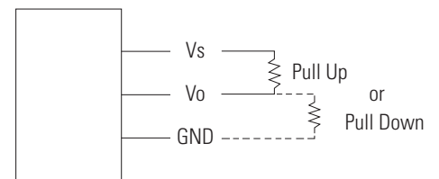
Figure 9. Output Load
