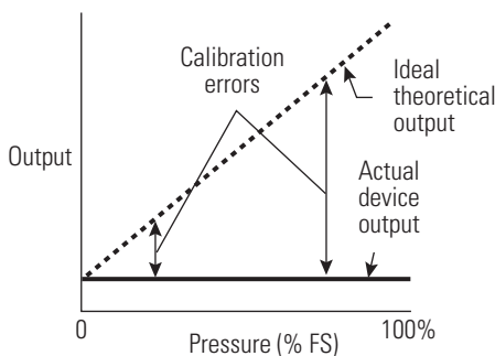
Figure 4. A useless pressure sensor with excellent “accuracy” (linearity, hysteresis and repeatability)
