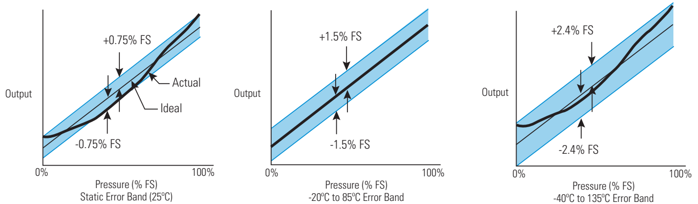
Figure 8. Error band at Different Temperature Ranges
