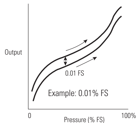
Figure 7. Repeatability
